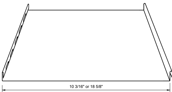
Panel Profile
