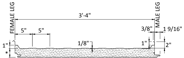
* ROOF PANEL THICKNESS: 3 1/4", 4", 5" or 6"
