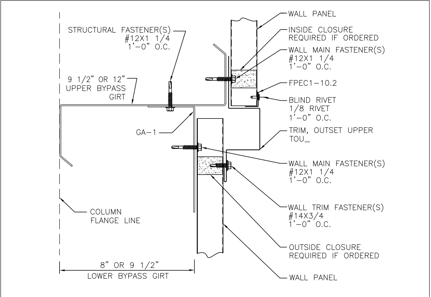
UPPER OUTSET GIRT TRANSITION (BYPASS / BYPASS) BYPASS UPPER GIRT TO BYPASS LOWER GIRT CONDITION
