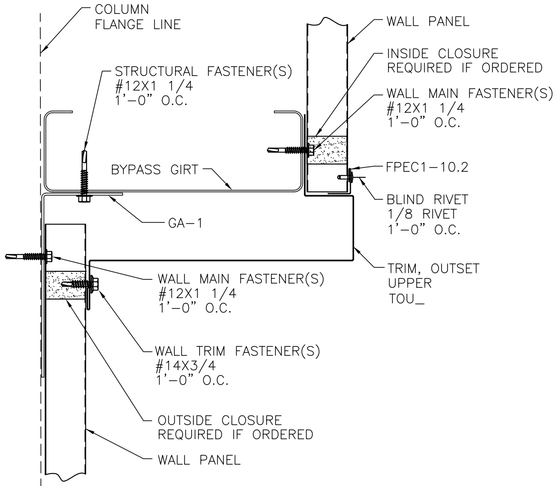
UPPER OUTSET GIRT TRANSITION (BYPASS / FLUSH) BYPASS UPPER GIRT TO FLUSH LOWER GIRT CONDITION
