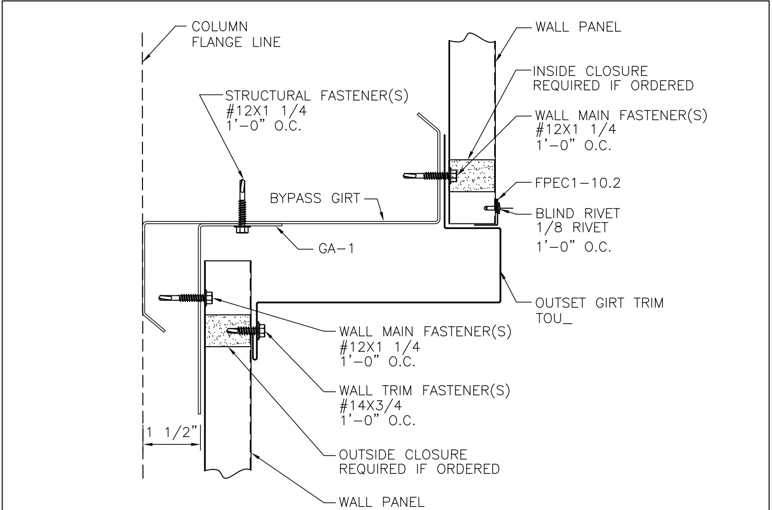
UPPER OUTSET GIRT TRANSITION (BYPASS / INSET) BYPASS UPPER GIRT TO INSET LOWER GIRT CONDITION
