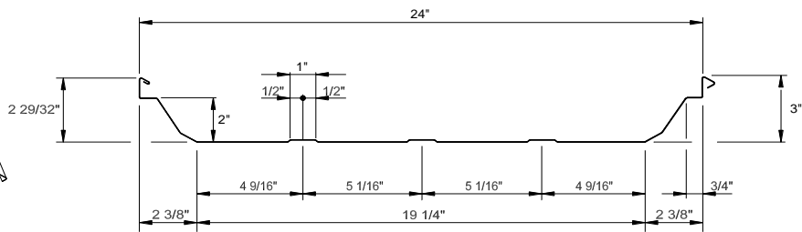
CROSS SECTION
